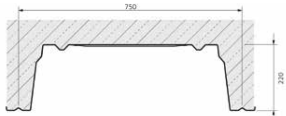
Composite floor parking
