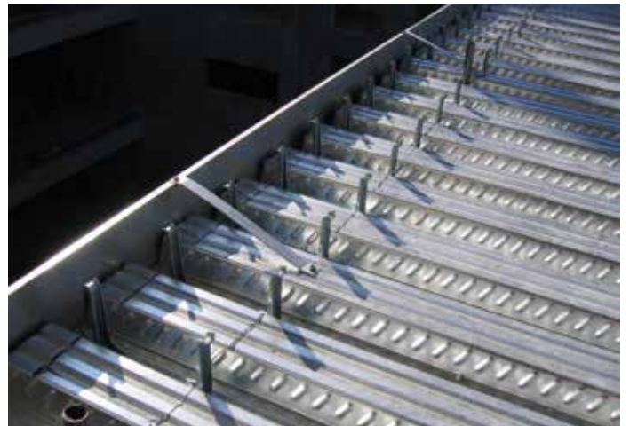
Edge trim with restraint strap and nailed shear studs
