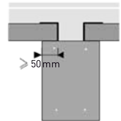
13 ■ Comply with minimum supports widths
